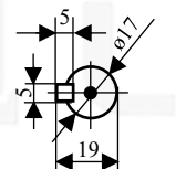
Output Shaft
