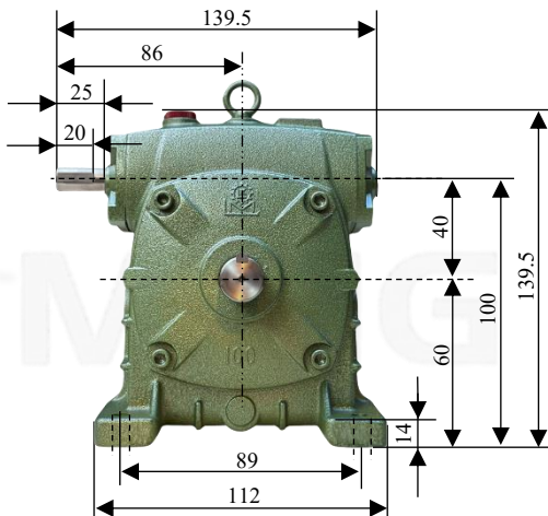
Output Shaft
