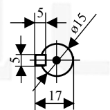
Output Shaft
