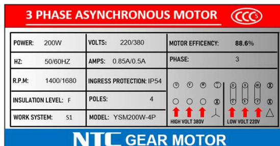
Nameplate
