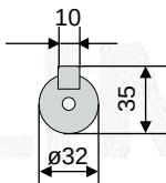
Output shaft
