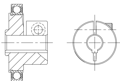
Collet + Keyway
